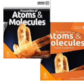
Properties of Atoms & Molecules
