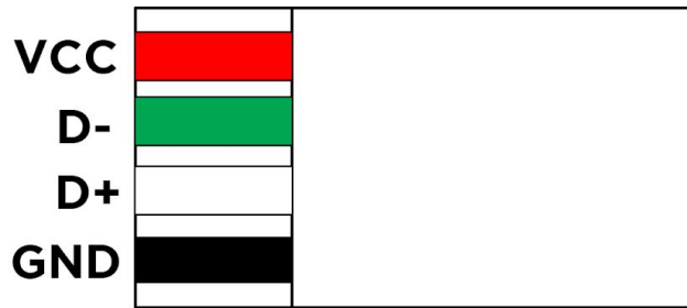
USB-MICRO
