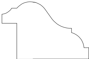
HM446 1 3/16" x 1 13/16"
