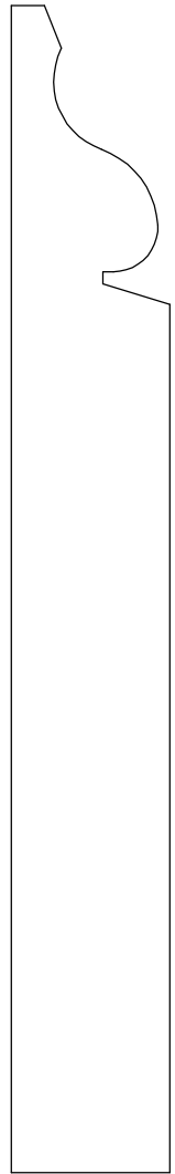
HM729 3/4" x 5 1/2"
