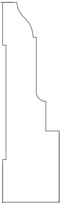
HM902 1" x 3 1/2"
