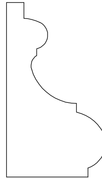
HM175 1 1/16" x 1 7/8"
