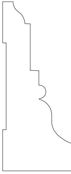
HM856 1 1/4" x 3 1/16"
