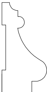
HM116 3/4" x 1 1/2"
