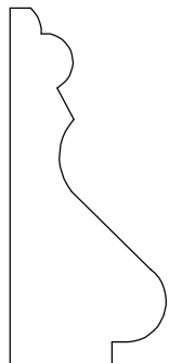
HM138 3/4" x 1 23/32"
