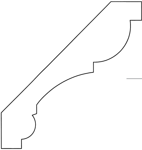
HM646 3/4" x 3 3/4"
