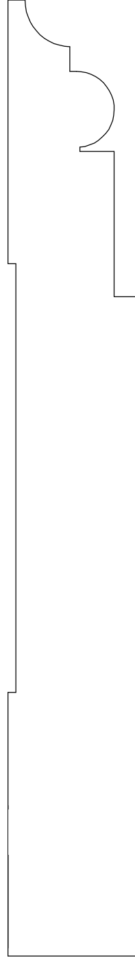
HM782 1" x 7 1/4"
