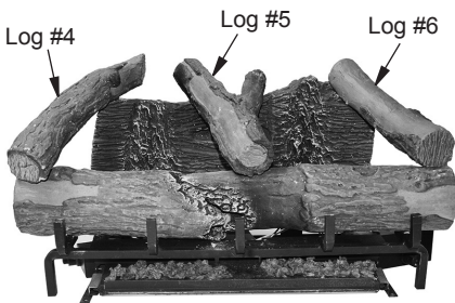
Figure 21 - Installing Logs #4, #5 and #6
