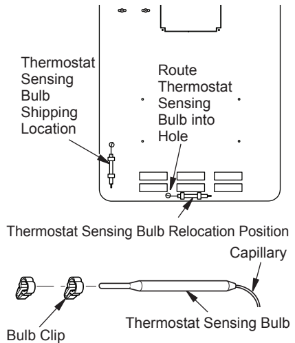
Figure 6 - Moving Thermostat Sensing Bulb
