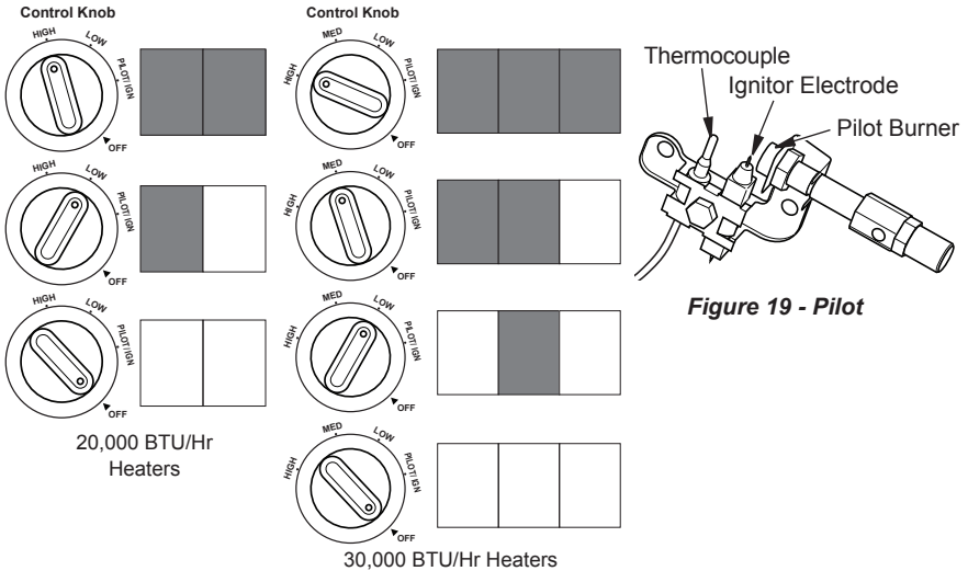
Figure 18 - Burner Patterns
