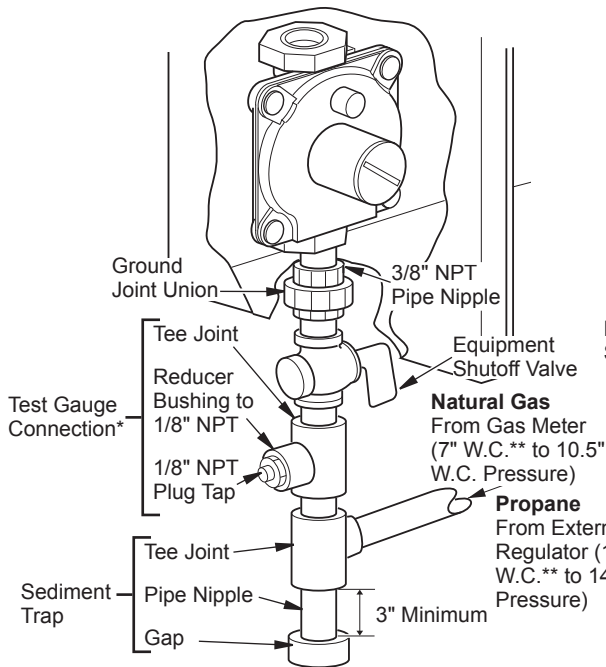
Figure 12 - Gas Connection
