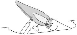
Figure 23 - Correct Pilot Flame Pattern
