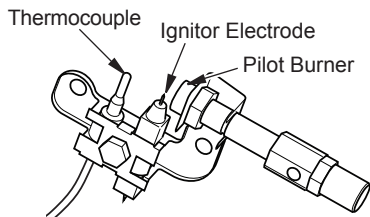
Figure 21 - Pilot
