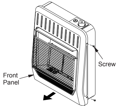
Figure 5 - Removing Front Panel
