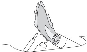
Figure 24 - Incorrect Pilot Flame Pattern
