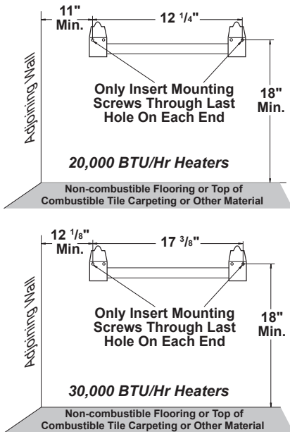
Figure 7 - Mounting Bracket Clearances
