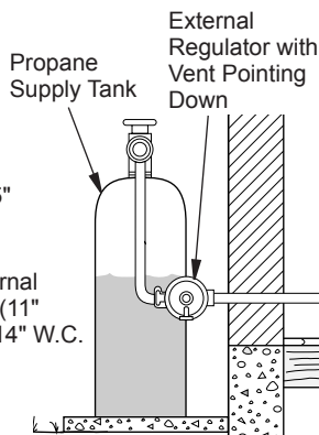
Figure 13 - External Regulator with Vent Pointing Down
