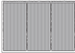
Figure 25 - Correct Burner Flame Pattern
