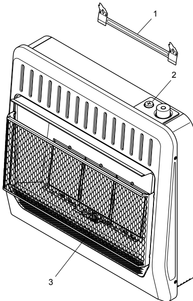
30,000 BTU/Hr Heater Shown
