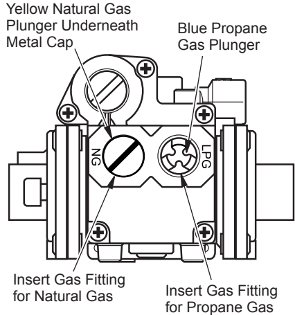
Figure 12 - Gas Regulator
