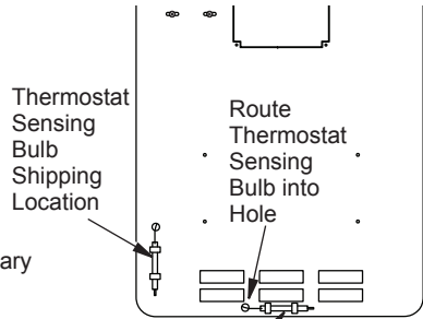
Thermostat Sensing Bulb Relocation Position
