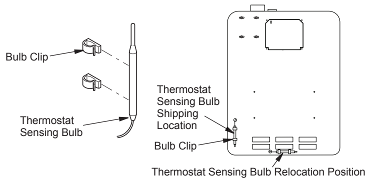
Figure 7 - Moving Thermostat Sensing Bulb Infrared Heaters Only
