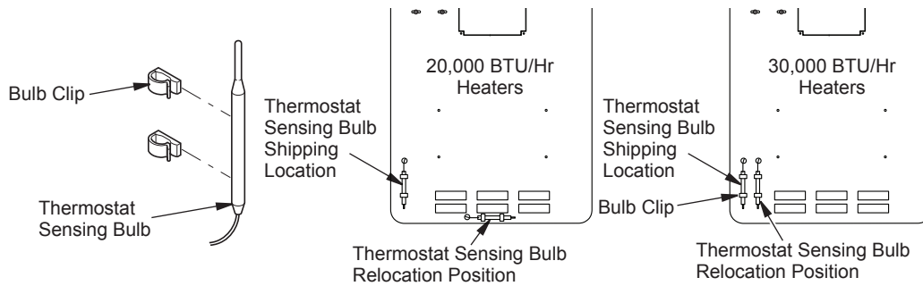
Figure 6 - Moving Thermostat Sensing Bulb Blue Flame Heaters Only
