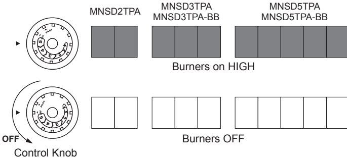
Figure 21 - Burner Patterns
