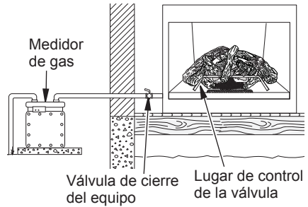
Figure 17 - Suministro de gas natural
