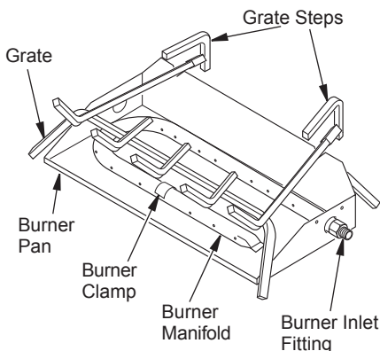
Figure 1 - Product Identification (WAN24LA Shown)
