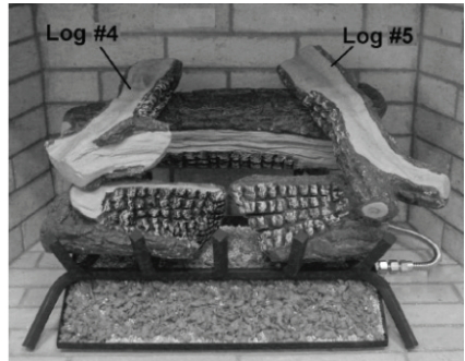
Figure 18 - Installing Top Logs #4 & #5
