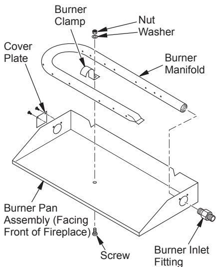
Figure 3 - Installing Burner
