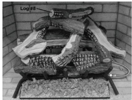
Figure 20 - Installing Top Log #8
