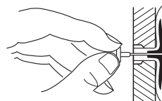
Figure 11 - Popping Open Anchor Wings For Thin Walls
