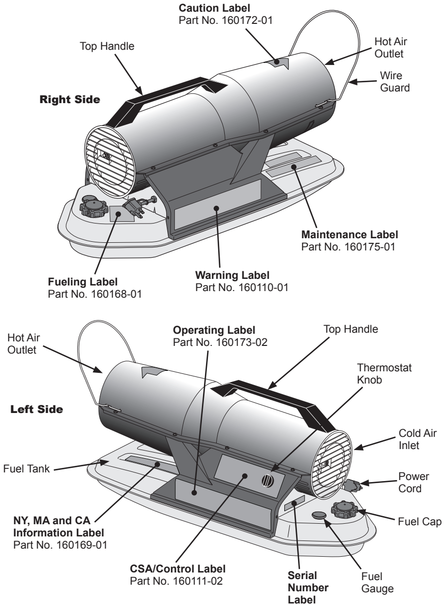
Figure 2 - Product Identification & Label Locations
