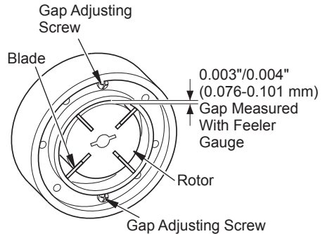
Figure 18 - Gap Adjusting Screw Locations
