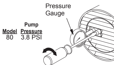
Figure 10 - Adjusting Pump Pressure
