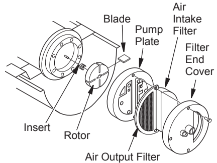
Figure 17 - Rotor Location
