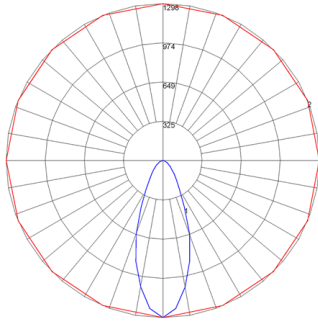
Maximum Candela = 1298.097 Located At Horizontal Angle = 0, Vertical Angle = 0 # 1 - Vertical Plane Through Horizontal Angles (0 - 180) (Through Max. Cd) # 2 - Horizontal Cone Through Vertical Angle (0) (Through Max. Cd)
