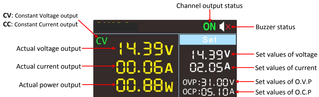
Figure 2-3 User Interface
