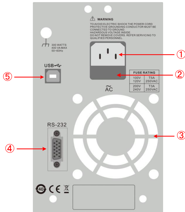
Figure 2-2 Rear Panel Overview
