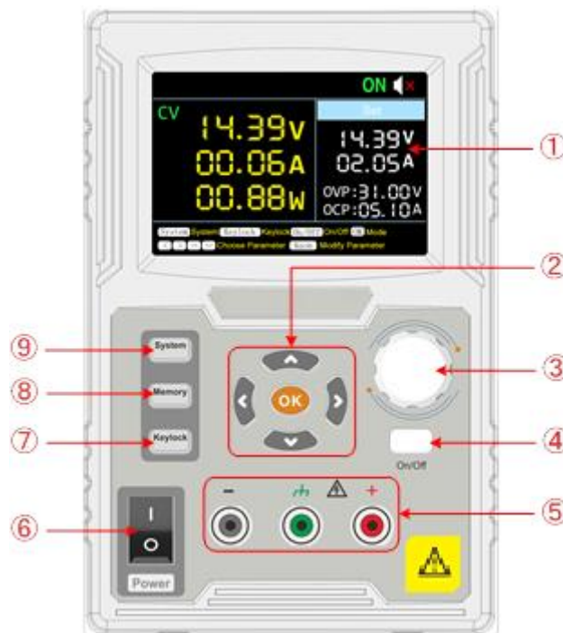
Figure 2-1 Front Panel Overview
