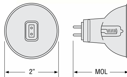
GU5.3
