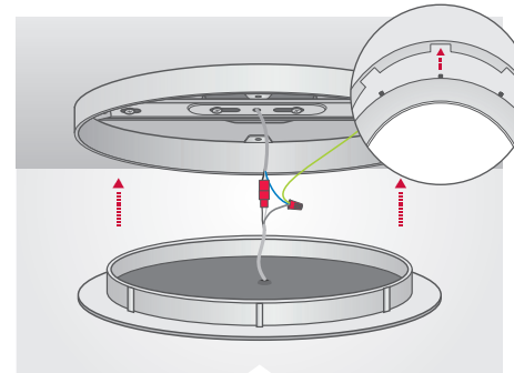
STEP 8: Raise the Lamp Unit up into the Mounting Bracket, push/feed the electrical wires up through the center hole into the junction box.
