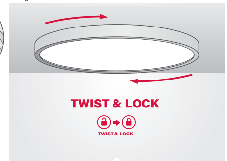
STEP 9: TWIST & LOCK (1)-(1) the Lamp Unit into the Mounting Bracket in the "Lock" direction to match up alignment arrows (1-2).
