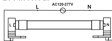
Figure 1a. - Double-Ended connection
