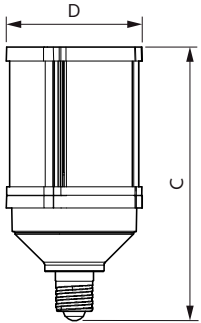
Corn lamp LED 27W E26 840 CL
