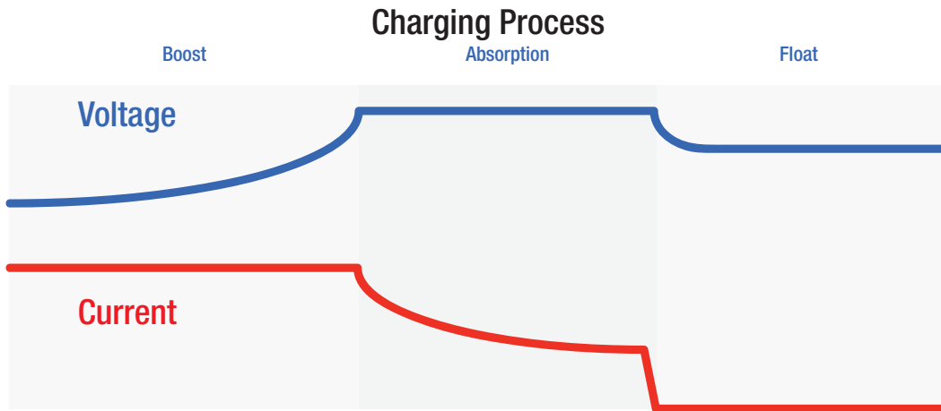
Figure 1.3.3.1 - Charging Process
