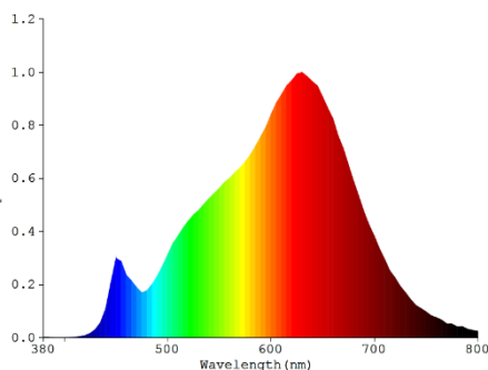
Spectral power distribution (2700K)
