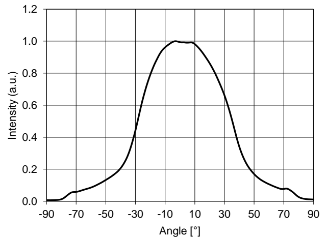
TYPICAL SPATIAL DISTRIBUTION (T A = 25°C, I F = 60 mA)
