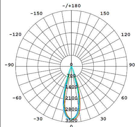
Distribution diagram (3000K 30°)
