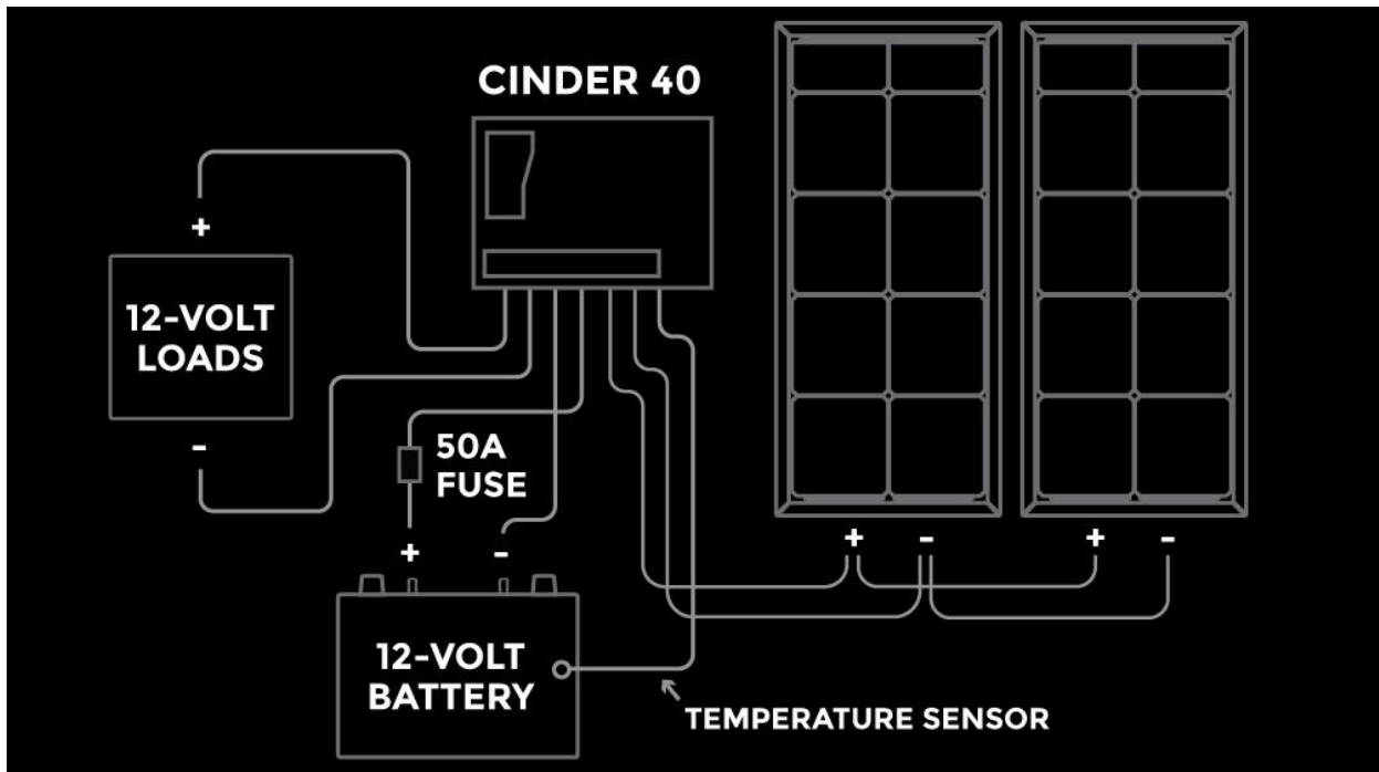
Figure 5: 12-Volt Installation Diagram
