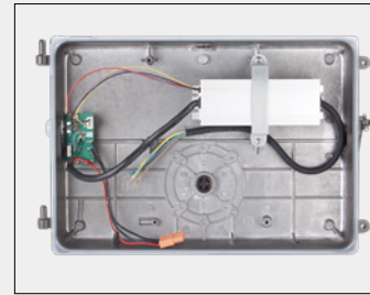
High Quality Driver Multi Voltage 100-277V/347V
