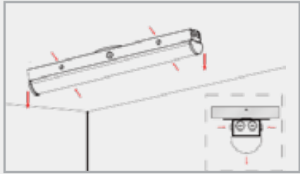
Surface-mounted
