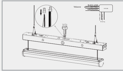
Suspending
