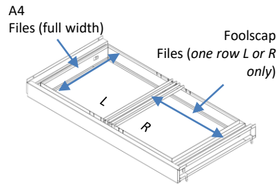
DT-POF-B/W Pull out suspension file rack Fits into Shelving clip slots W : 735mm D : 365mm H : 75mm Col: Black or White
