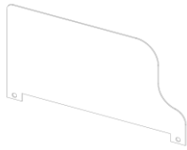
DT-DIVIDER-B/W Steel divider – Black or White Slots into slotted shelves W : 379mm H : 175mm 2mm thick metal plate Sold in sets of 5
