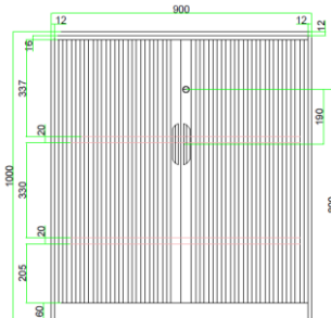
DT-1000-90-B/W 3 levels - Adjustable Recommended spacing: 1 st FFL : 205mm 2 nd FFL : 330mm 3 rd FFL : 337mm Shelves : 2 included
