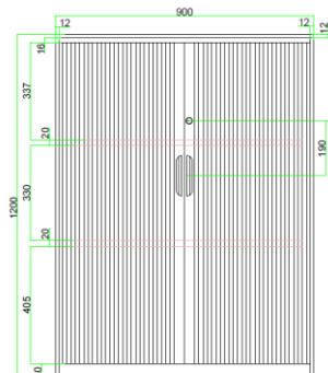
DT-1200-90-B/W 3 levels - Adjustable Recommended spacing: 1 st FFL : 405mm 2 nd FFL : 330mm 3 rd FFL : 337mm Shelves : 2 included
