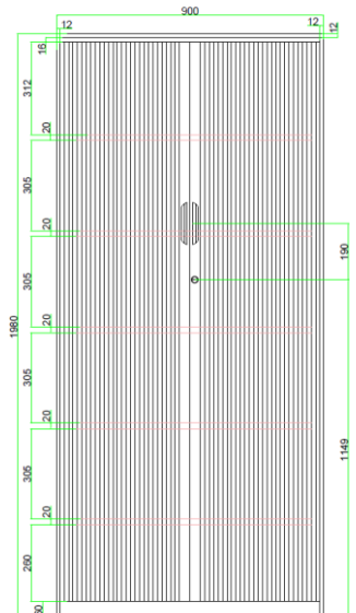
DT-H1980-90-B/W 5 levels - Adjustable Recommended spacing: 1 st FFL : 260mm 1-4 th FFL : 305mm 5 th FFL : 312mm Shelves : 5 included
