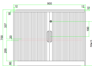
DT-700-90-B/W 2 levels - Adjustable Recommended spacing: 1 st FFL : 255mm 2 nd FFL : 337mm Shelves : 1 included
