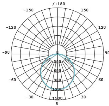
SL3247/40CW at 4000K
