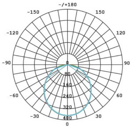
SL3247/25CW at 4000K
