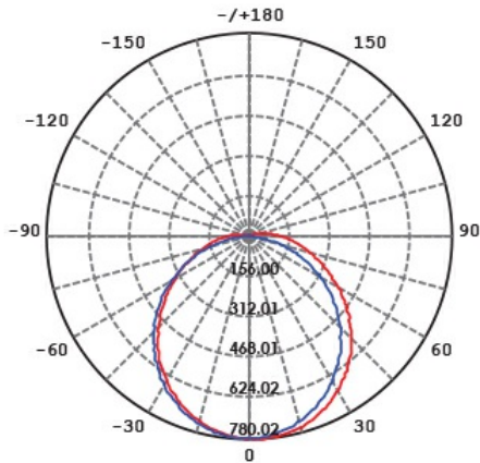
SL9709/60TC at 3000K
