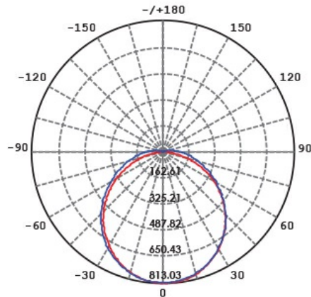
SL9709/120TC at 5700K
