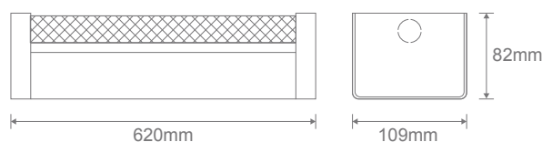
Internal ON/Off Sensor
