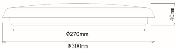
OYSDIM002-LINE DRAWINGS
