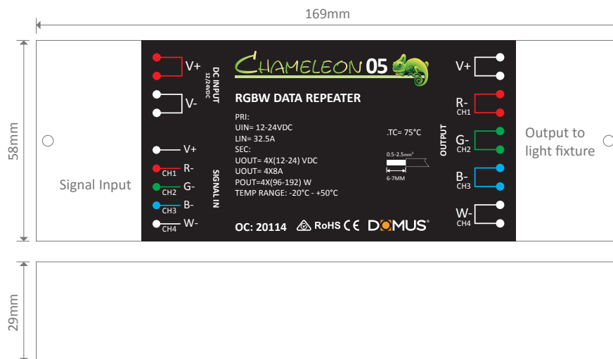
RGBW Colour Changing (Fig 1)
