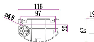
Back plate
