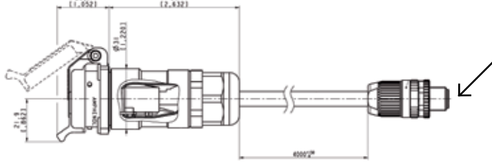
Part number: Kit 36530 - Length 4 m [13.12 ft]
