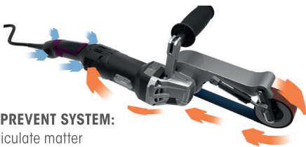
With DUST PREVENT SYSTEM: Ideal heat dissipation and motor protected from particulate matter
