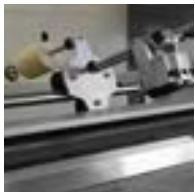
Double station: belt grinding and finishing in one machine
