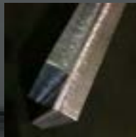
Removing oxide layer with wire brushes cross belts
