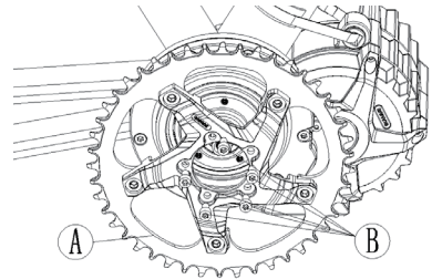
A Chainset
