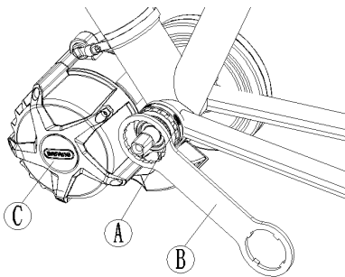
A Locking ring M33-PH1(B)
