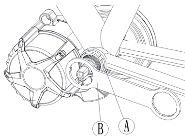
A Locking ring M33-A B Special tool
