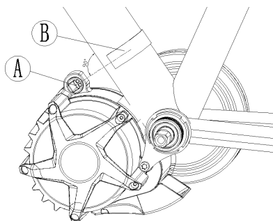
A Hoop set B Rubber washer
