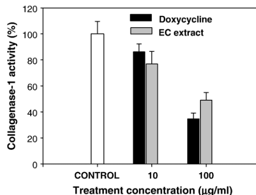
Fig. 3. Effect of EC extract on bacterial collagenase-1 activity tested using fluorometric assay. Bacterial collagenase-1 was reacted with 100 µg/ml and 10 µg/ml of EC for 18 h using doxycycline as the positive control. Fluorescence intensity, which represents bacterial collagenase-1 activity, was measured at 495/520 nm (excitation and emission). Error bars represent mean and S.D. from triplicate experiments after deduction of background values from raw values.
