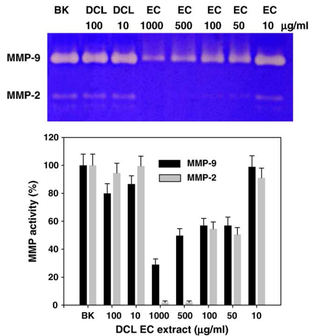
Fig. 6. Effects of EC extract on activities of MMP-2 and MMP-9 from HT1080 cells. Cells were treated with 10 ng/ml of PMA under serum-free conditions to induce MMP expressions. After 3 days of incubation, conditioned media were reacted with various concentrations of EC extract for 1 h, and then gelatin zymography was performed. Doxycycline (DCL) was used as the positive control. Lower panel represents respective relative enzyme activities as percent of blank group.
