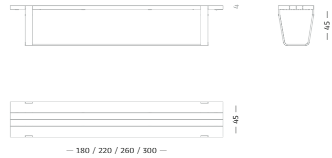
BB 12 Clamp® Outdoor Sitzbank / Bench
