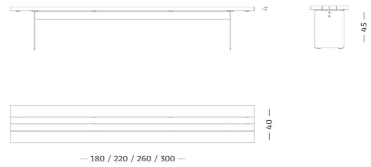
SC 48 Outdoor Sitzbank / Bench
