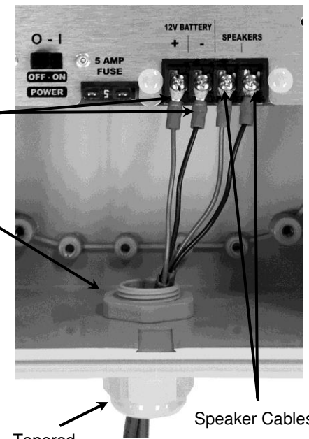
Tapered Cinch Nut Figure 6
