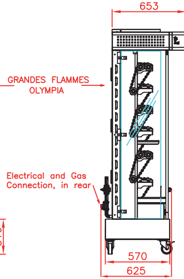
Side view Rotisserie with roof and base on casters
