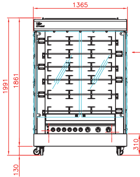
Front view Rotisserie with roof and base on casters
