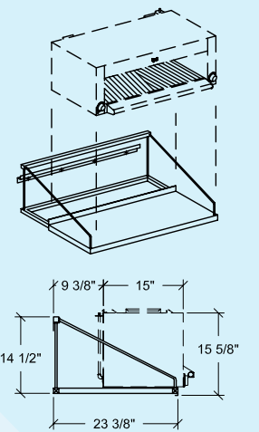
EXTENDED WALL MOUNT
