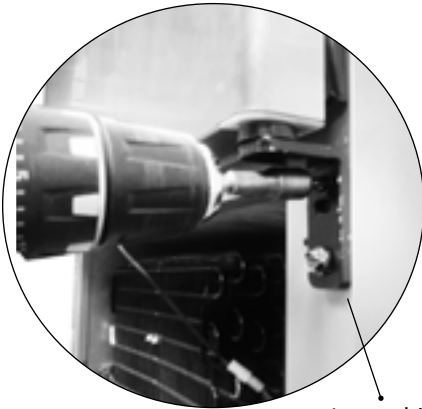
Lower hinge
