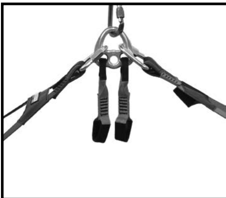
Contracted (Rail work) Position
