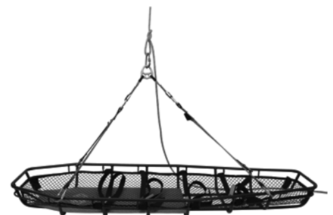
Standard Rigging
