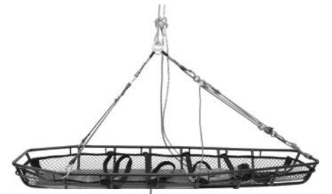
Tilt/ Lift Rigging
