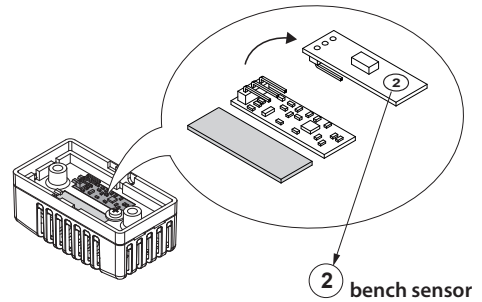
2 bench sensor
