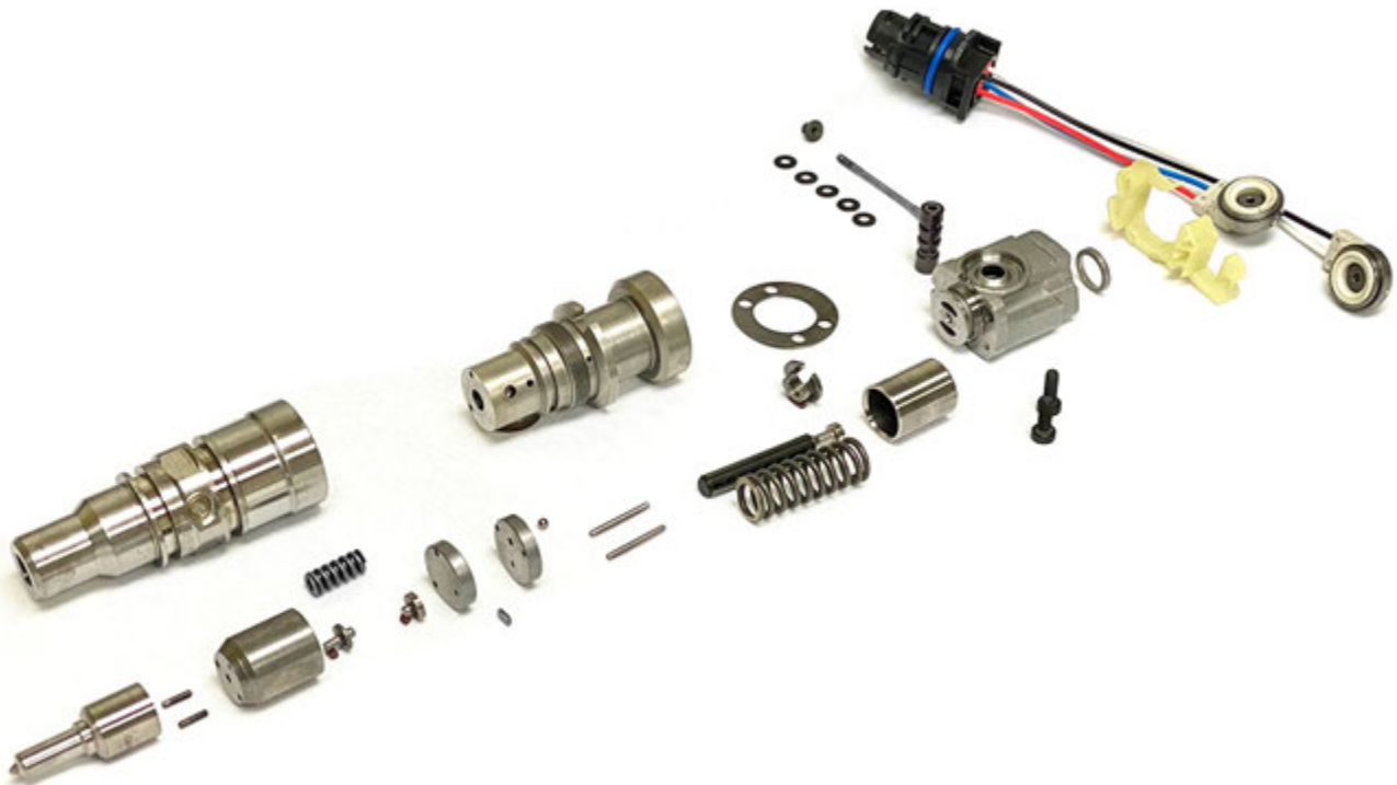
G2.8 INJECTOR PARTS EXPLODED VIEW
