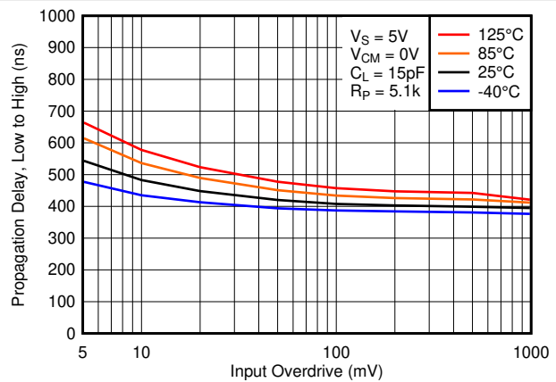
Figure 7-31. Low to High Propagation Delay vs. Input Overdrive Voltage, 5V
