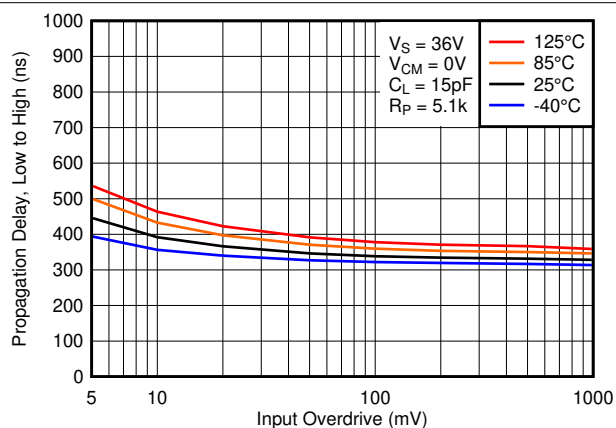
Figure 7-35. Low to High Propagation Delay vs. Input Overdrive Voltage, 36V
