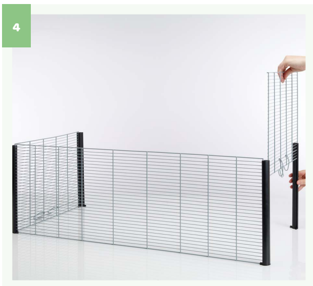
Slide the second side panel (l) into the final profile. Make sure the closure is facing outwards.
