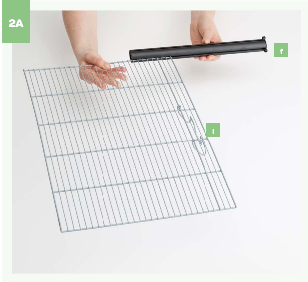
Slide one side panel (l) into two profiles (f).
