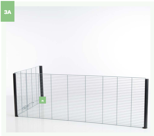
Slide the back panel (n) in the third profile. Make sure that the vertical wires of the back panel and the closure of the side panel are facing outwards.
