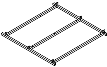
Bottom-Back Frame
