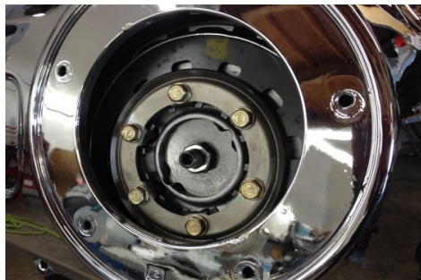
Non Slipper Clutch, 6 Studs Style
